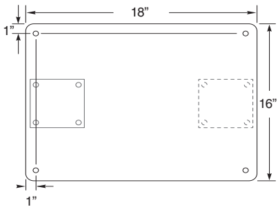
3486WM Leveling/Mounting Board
