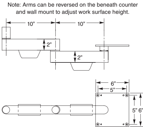
3486BC and WM Mounting Arm
