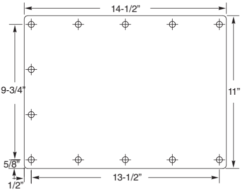
3486BC Heavy Duty Mounting Plate
