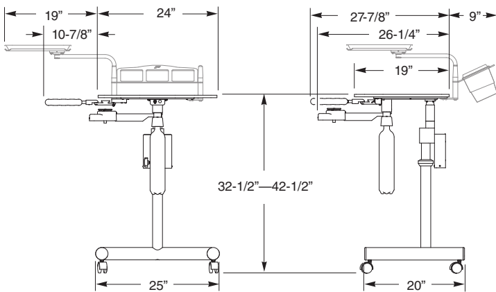
3486MC Mobile Cart
