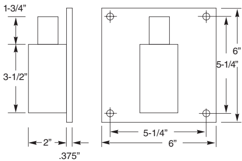
3486WM Wall Mount Hub
