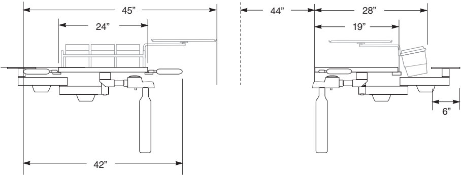
3486WM Wall Mount Hub
